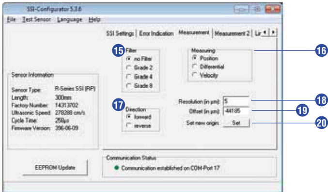
Fig. 33: Temposonics SSI-Configurator, Measurement
