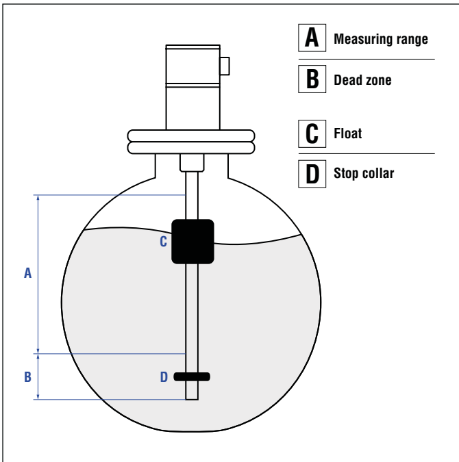
Fig. 20: Liquid level measurement
