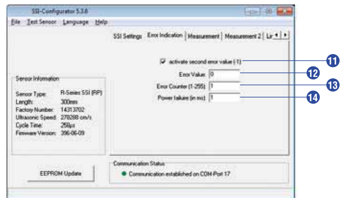
Fig. 32: Temposonics SSI-Configurator, Error Indication
