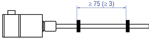
Fig. 19: Minimum distance between magnets for differentiation measurement
