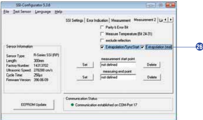
Fig. 35: Temposonics SSI-Configurator, Measurement 2, choose “synchronous mode 3”
