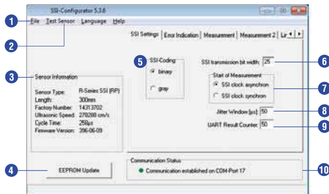
Fig. 30: Temposonics SSI-Configurator, SSI Settings
