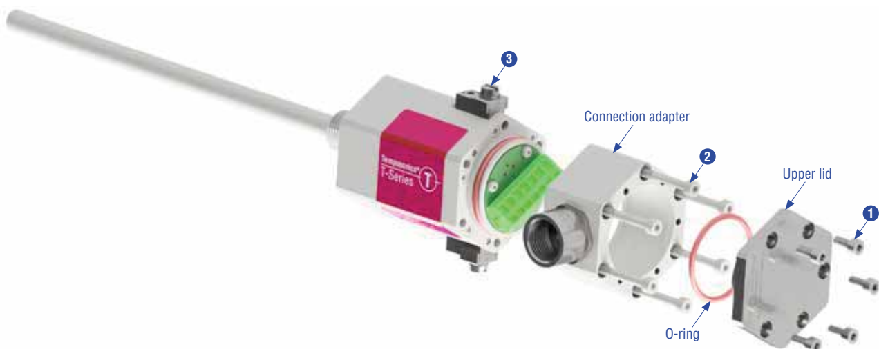
Fig. 6: Temposonics® TH exploded view drawing
